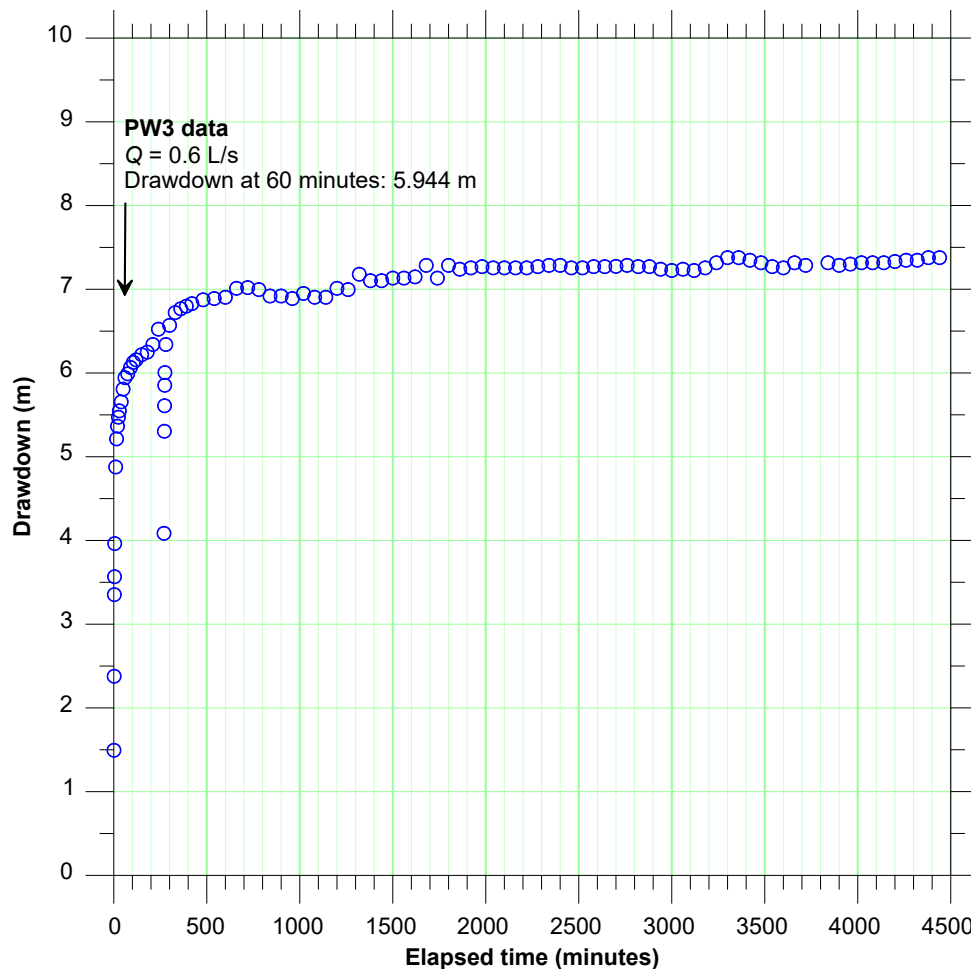
Figure 13. Drawdown record for the PW3 pumping test
