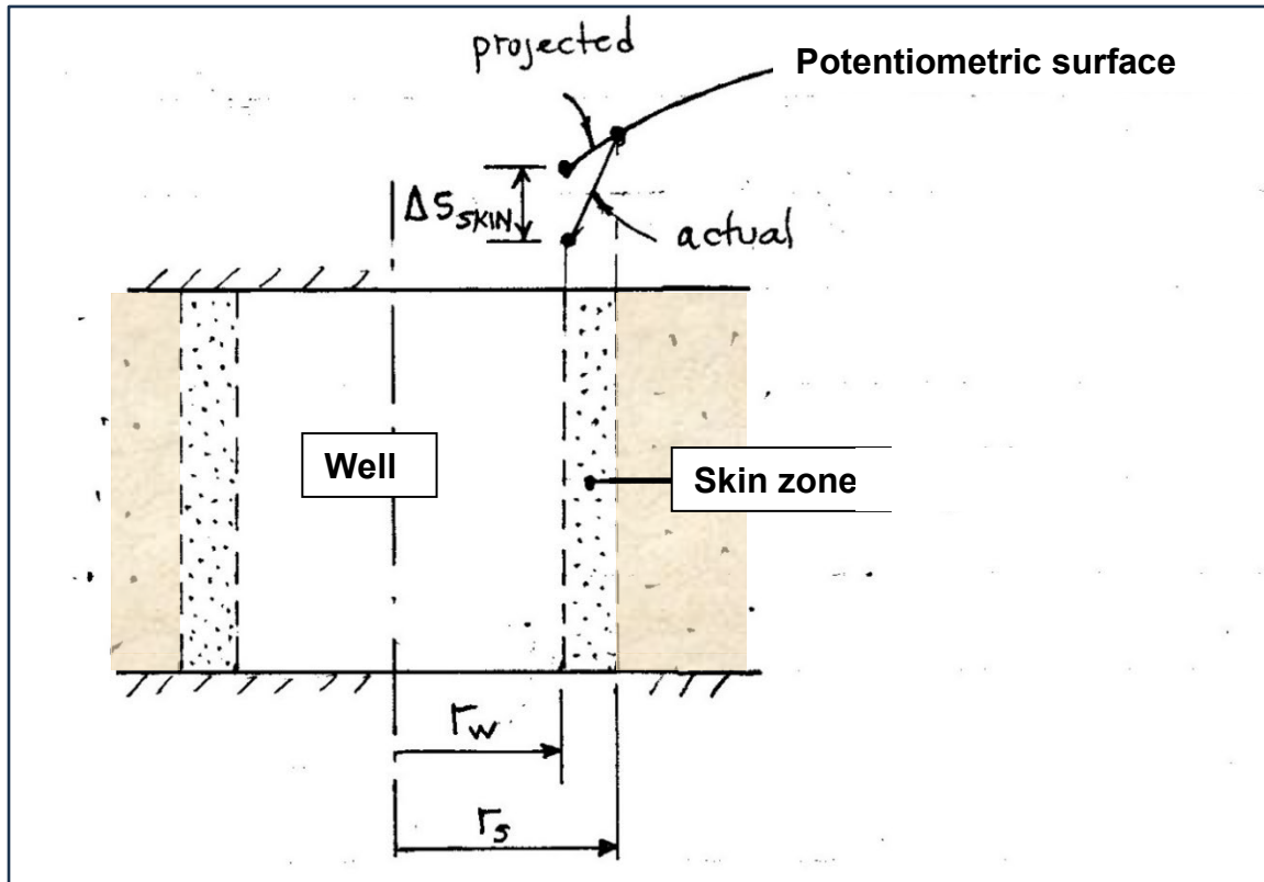
Figure 15. Schematic cross-section of a well surrounded by a skin zone
