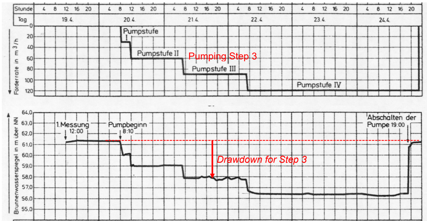
Figure 5. Data from municipal well testing, Linnich, Germany (Data from Langguth and Voigt, 1980)
