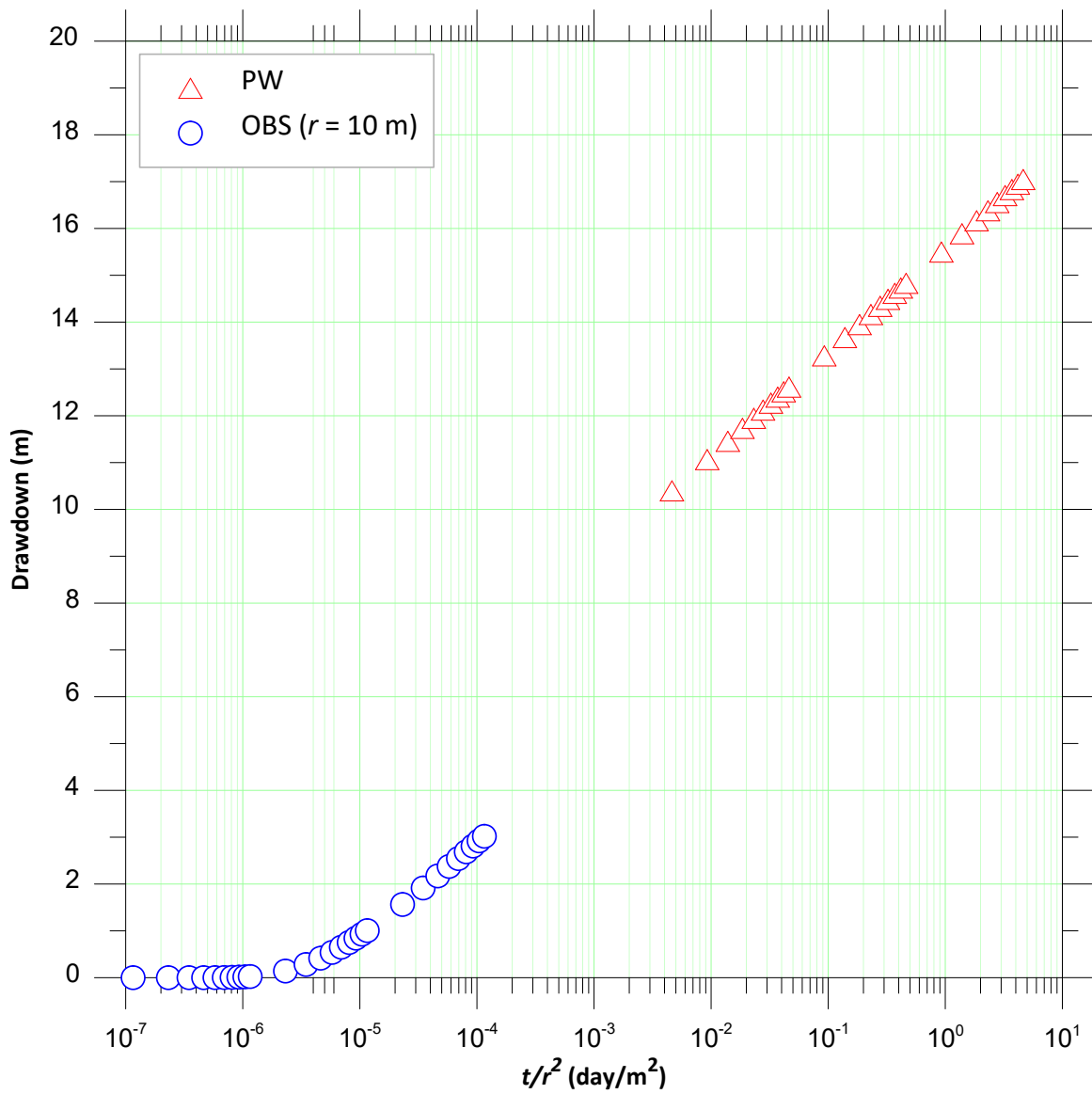
Figure 34. Composite plot for the pumping well and observation well
