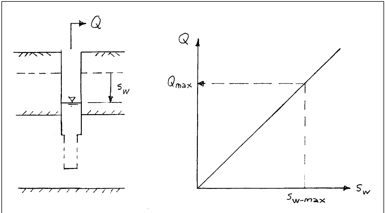
Figure 4. Estimation of the capacity of well with a constant specific capacity
