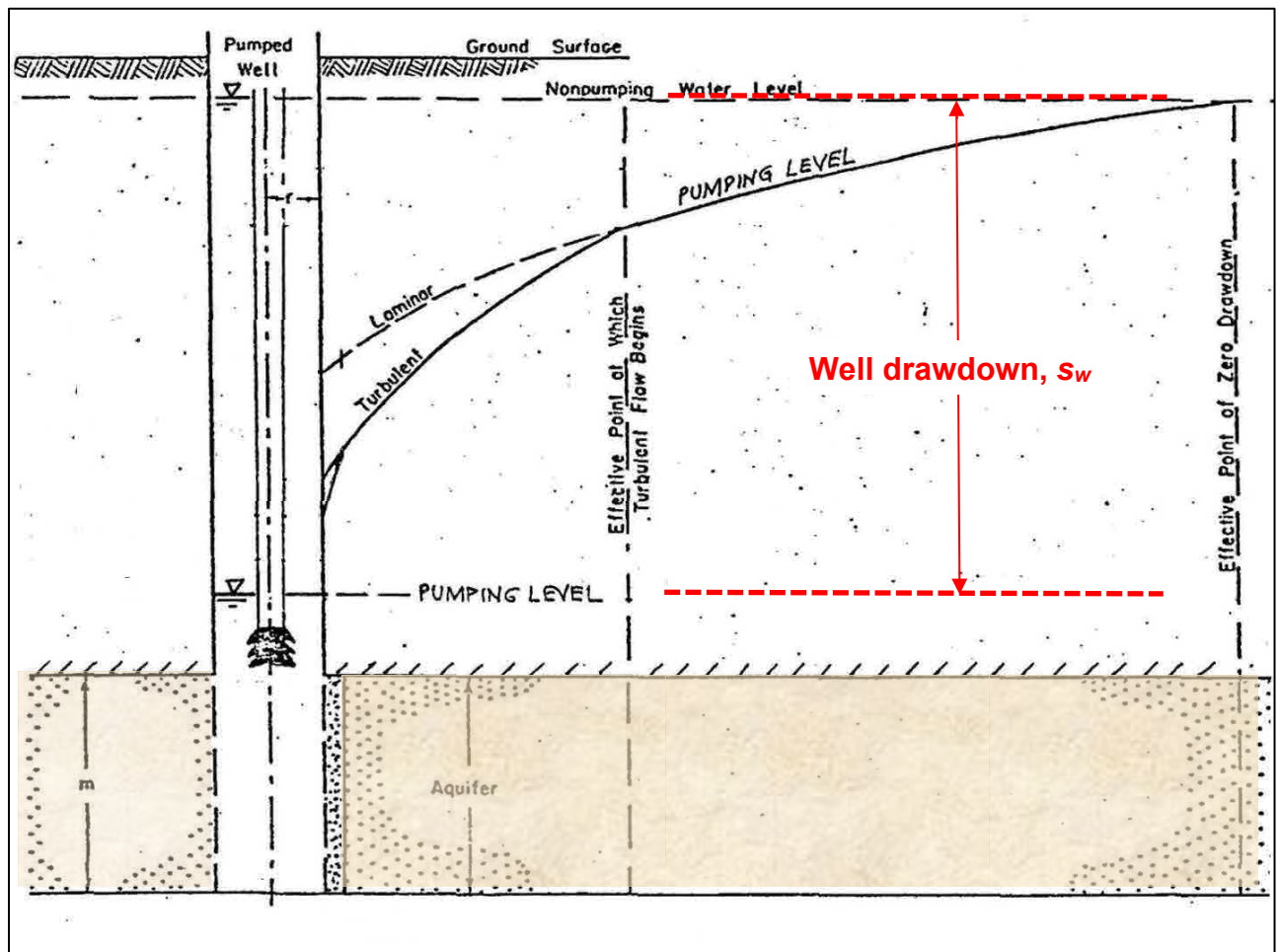
Figure 1. Drawdown in a pumping well Adapted from Bruin and Hudson (1955)
