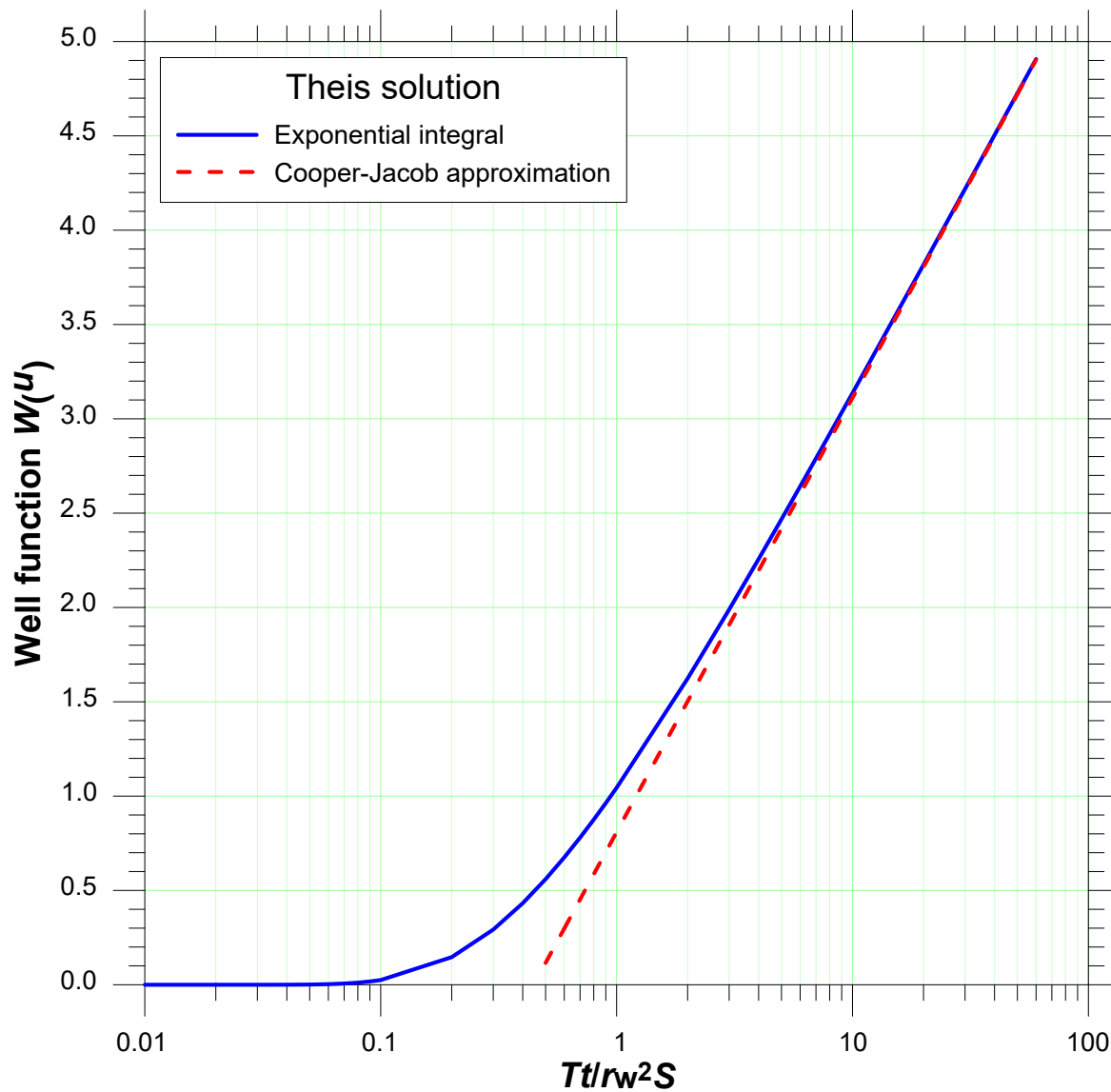
Figure 9. Theis well function and its approximation
