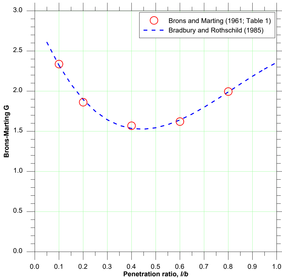
Figure 17. Values of the Brons-Marting function G for partially penetrating wells
