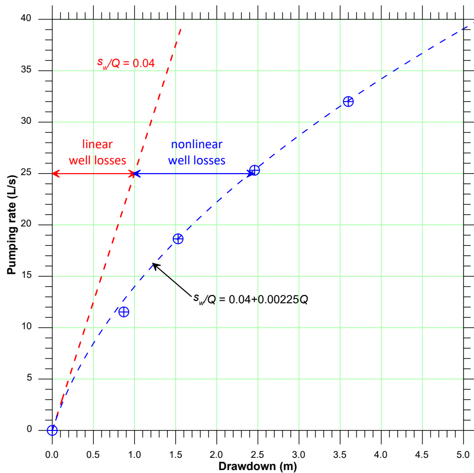
Figure 27. Specific capacity with inferred relation from the Hantush-Bierschenk plot
