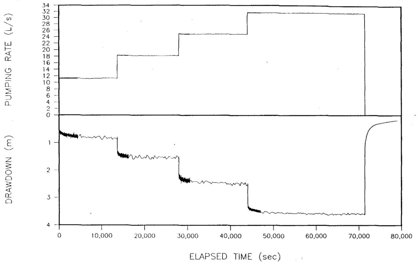
Figure 24. PW6/63 step test data
