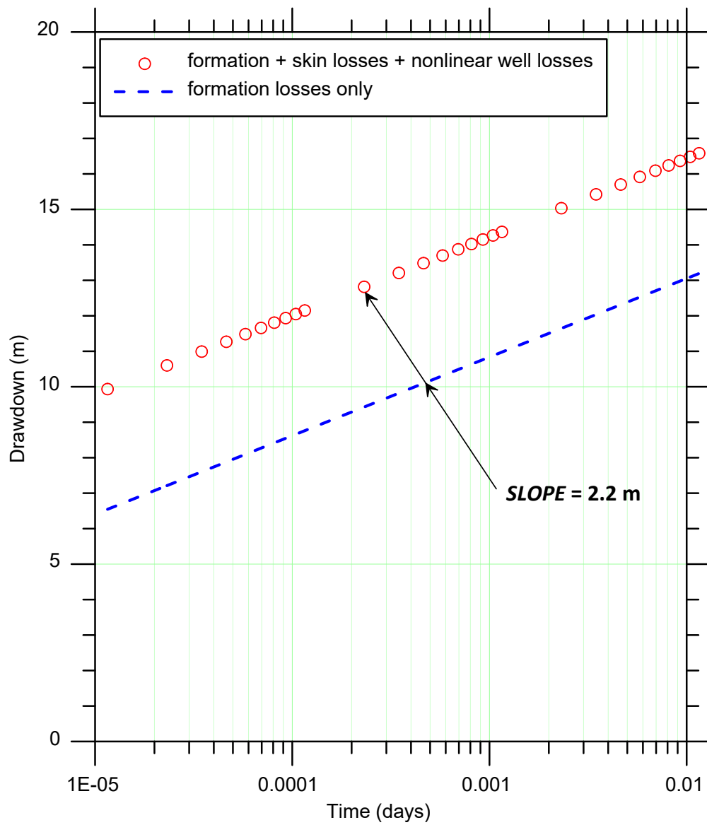
Figure 18. Drawdowns at the pumping well
