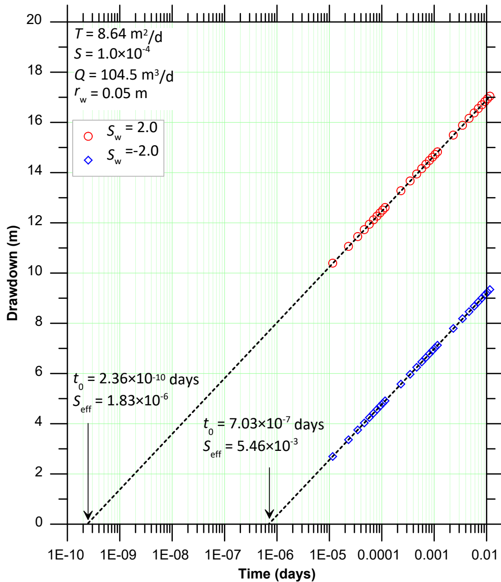
Figure 21. Example pumping well drawdowns with skin zones
