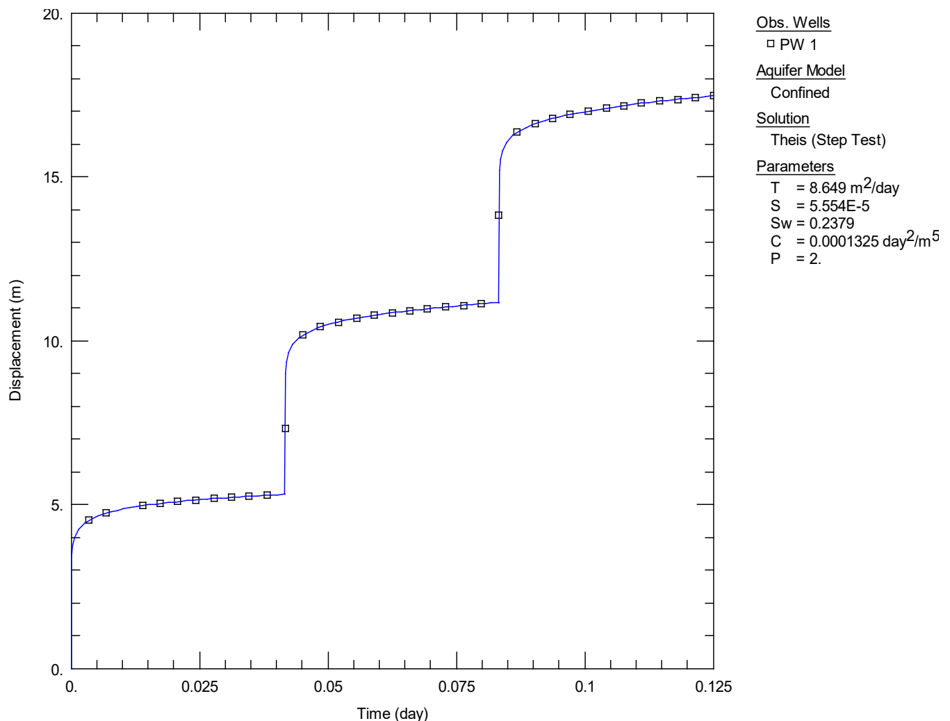
Figure 30. AQTESOLV match to hypothetical step test results
