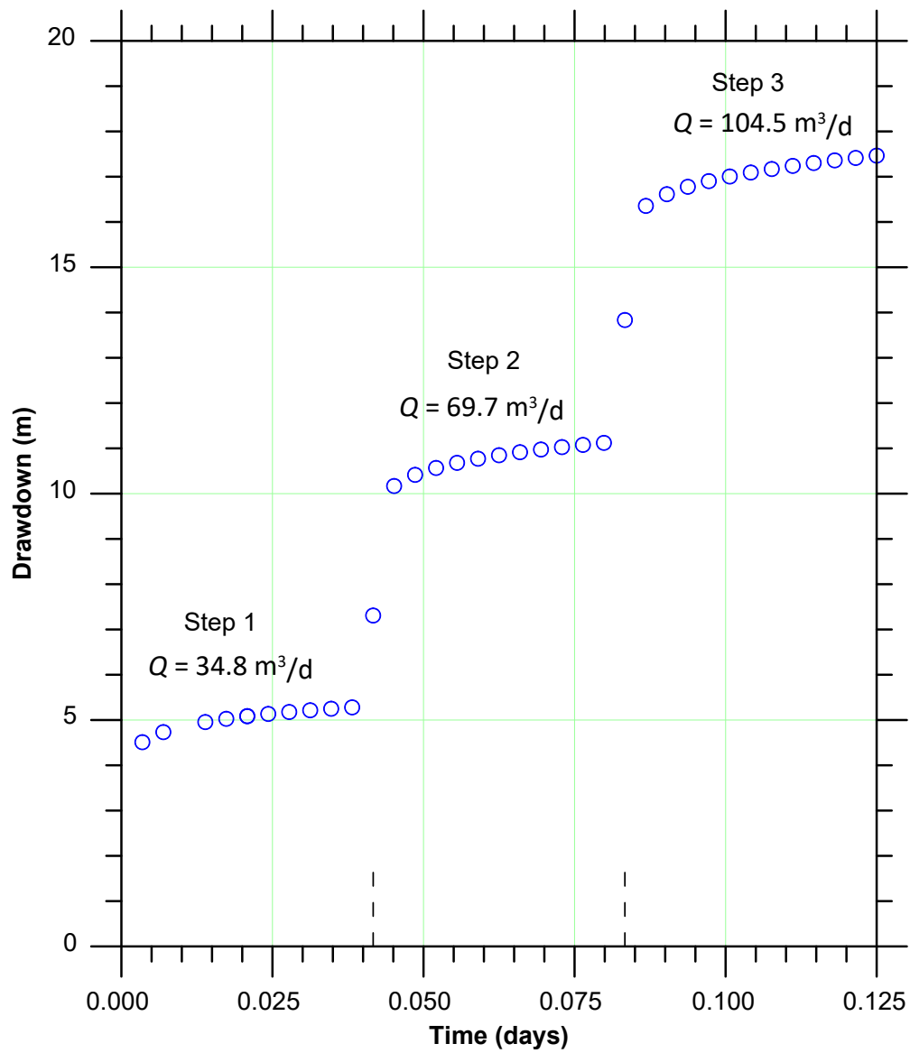
Figure 29. Pumping well drawdowns for a hypothetical step test
