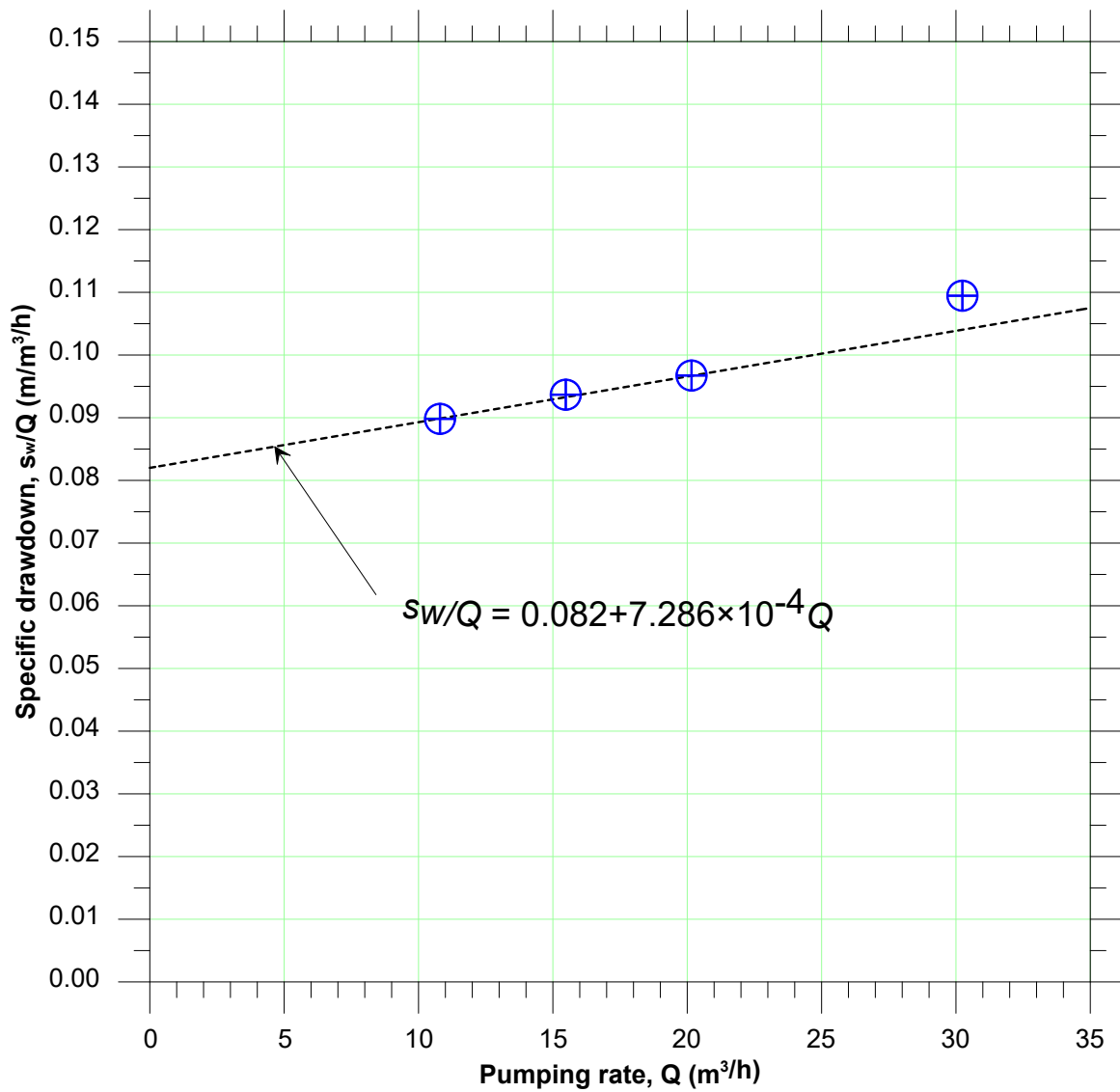
Figure 23. Hantush-Bierschenk plot, data from Figure 18
