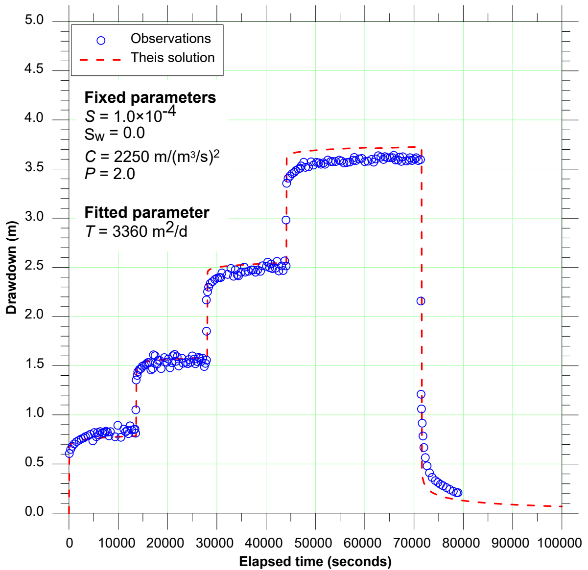
Figure 33. Match to the full transient drawdown record
