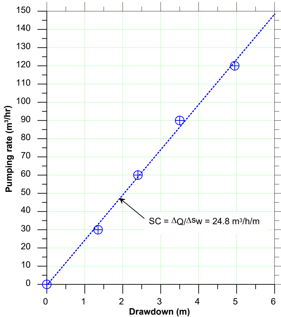
Figure 6. Reduced data from the Linnich step test
