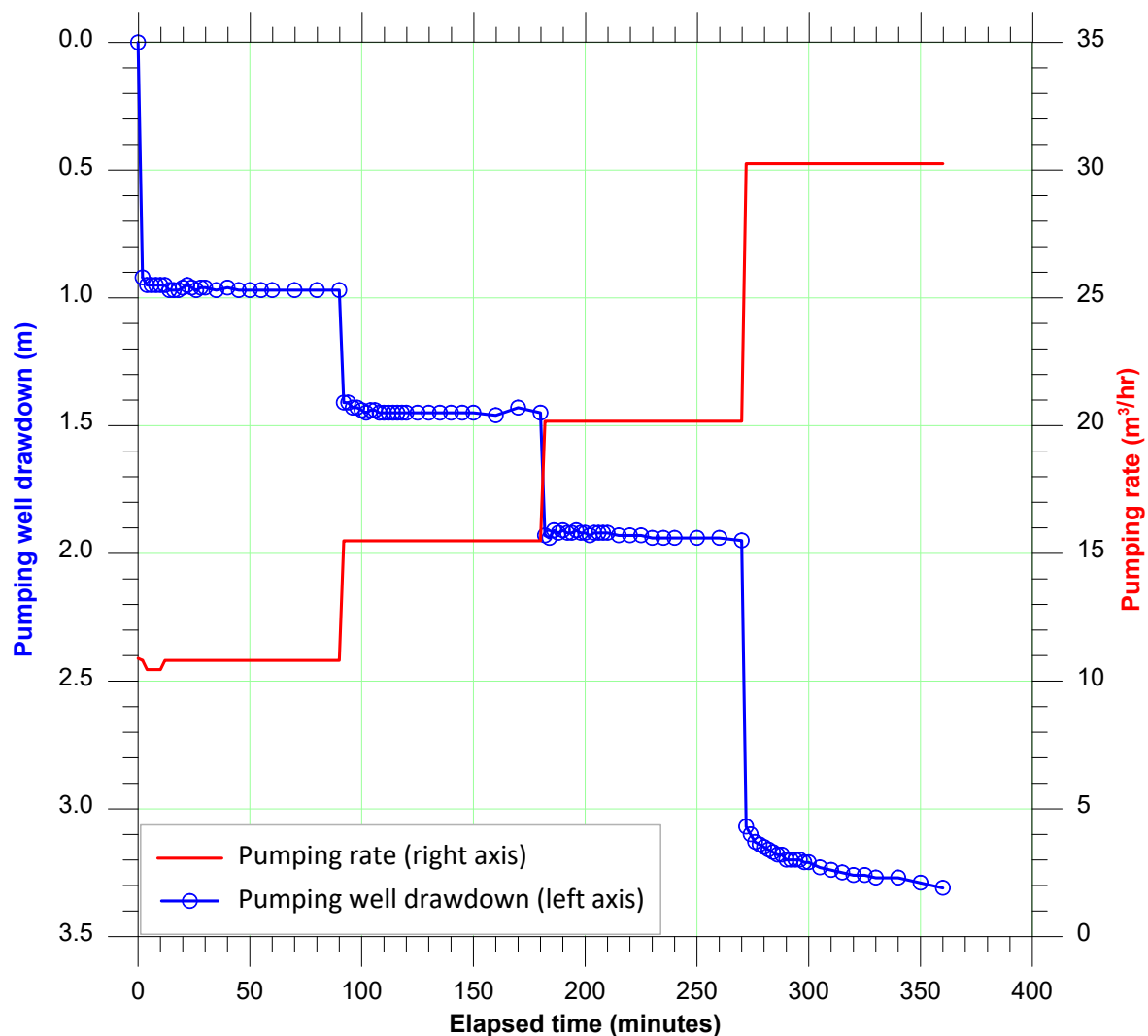
Figure 22. Example step test data
