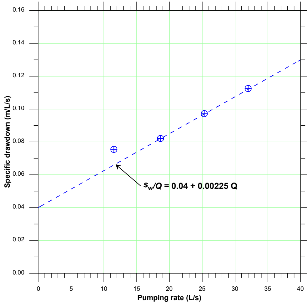
Figure 26. Specific drawdown vs. pumping rate
