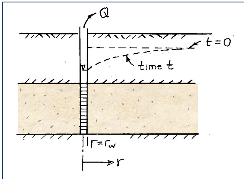
Figure 3. Idealization of the component of drawdown due to head losses in the formation
