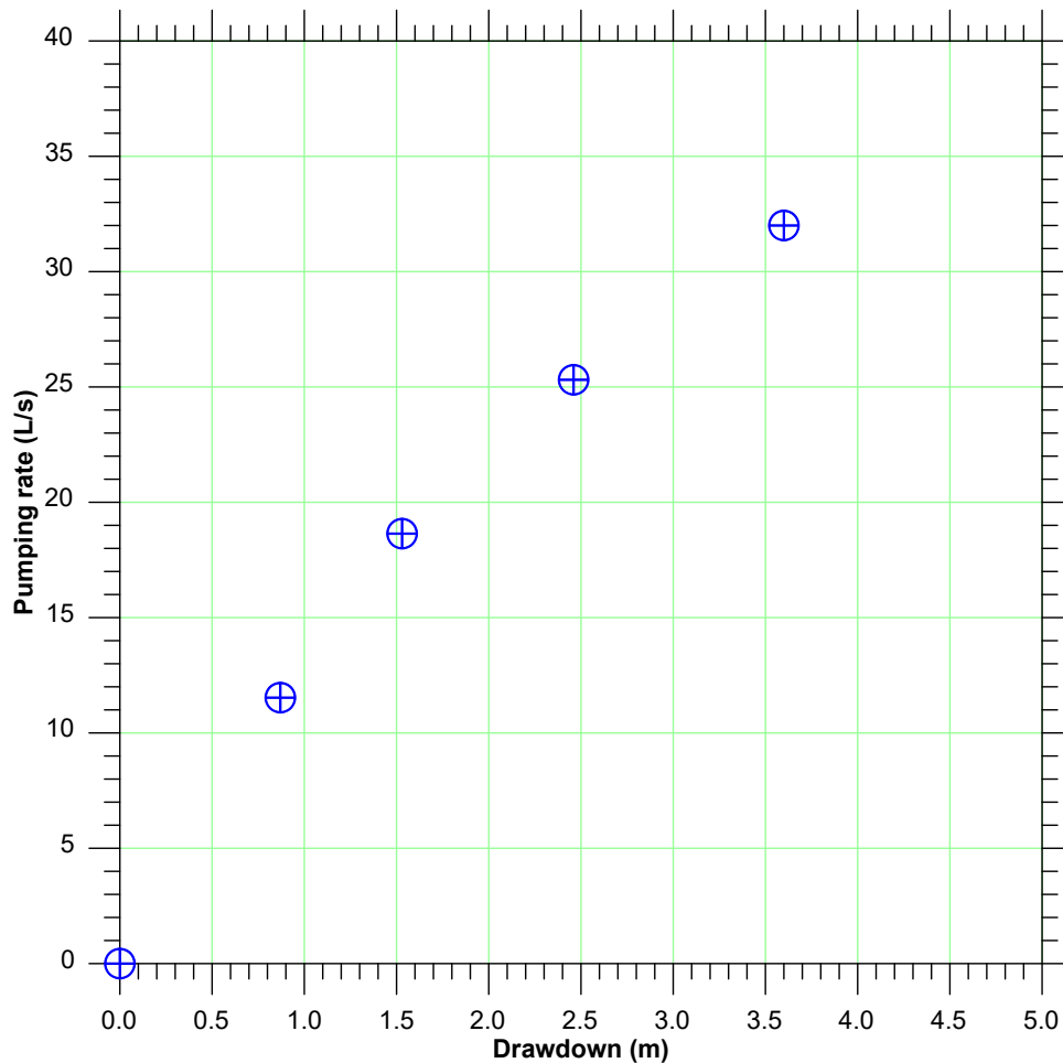
Figure 25. “Raw” specific capacity results
