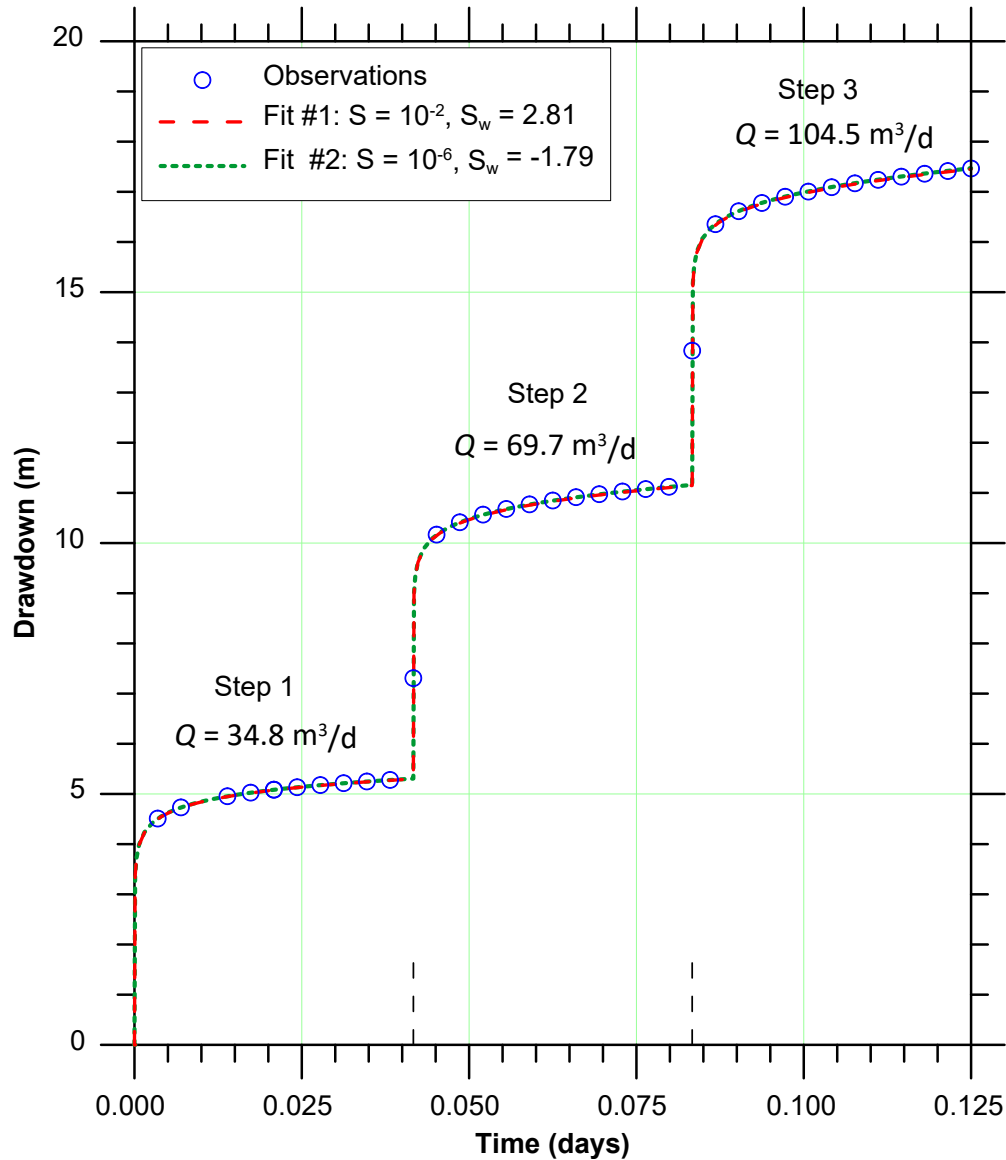
Figure 32. Alternative AQTESOLV matches to hypothetical step test results
