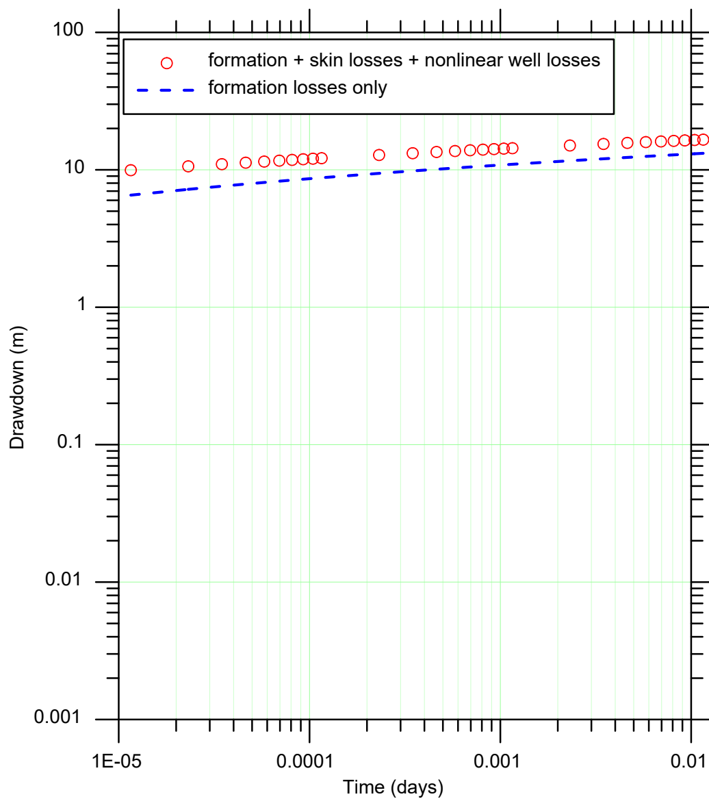
Figure 20. Drawdowns at the pumping well, log-log axes
