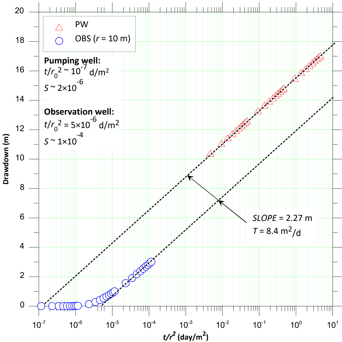
Figure 35. Cooper-Jacob analyses on the composite plot
