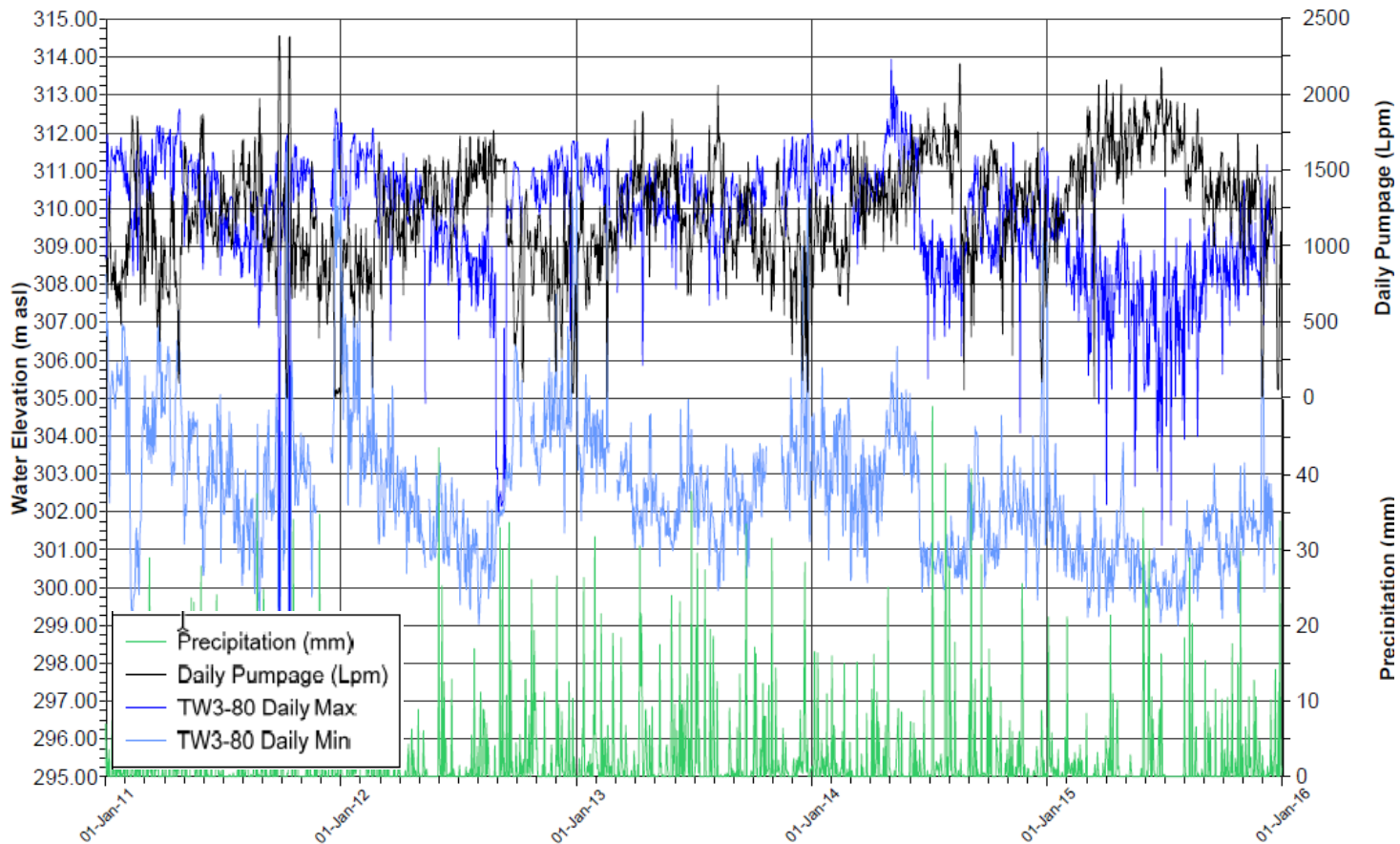
Figure 7. Performance record for an operating production well
