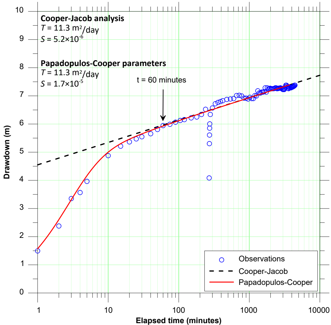
Figure 14. Rigorous analyses of the PW3 pumping test
