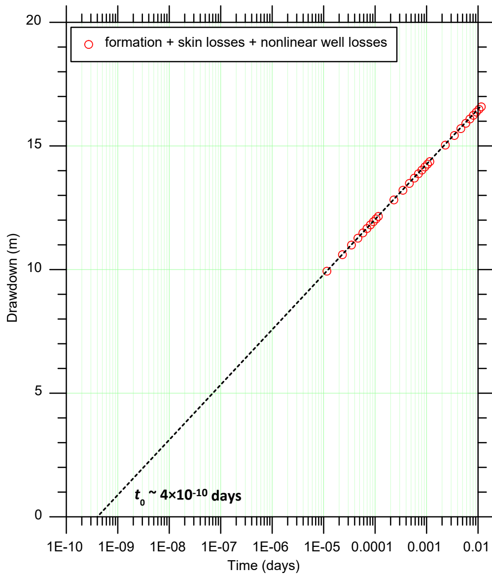
Figure 19. Drawdowns at the pumping well, with expanded time axis
