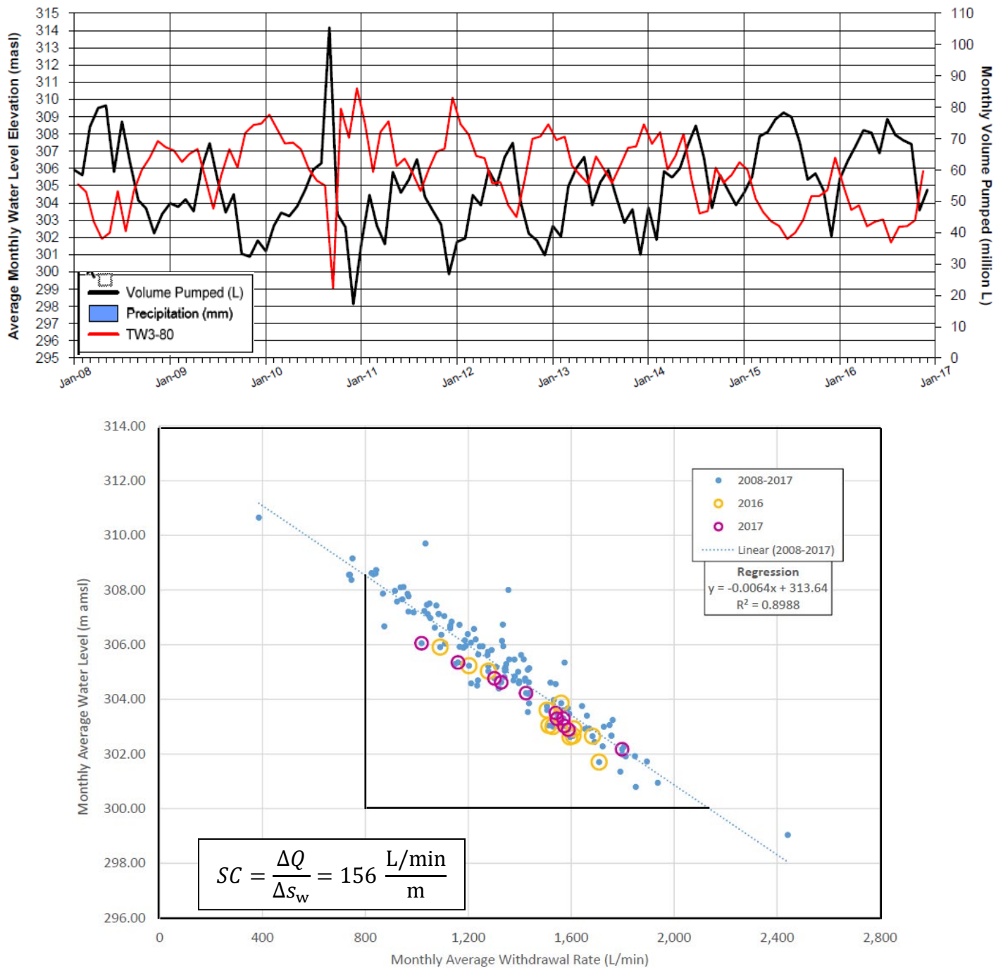
Figure 8. Monthly-average operating well performance data
