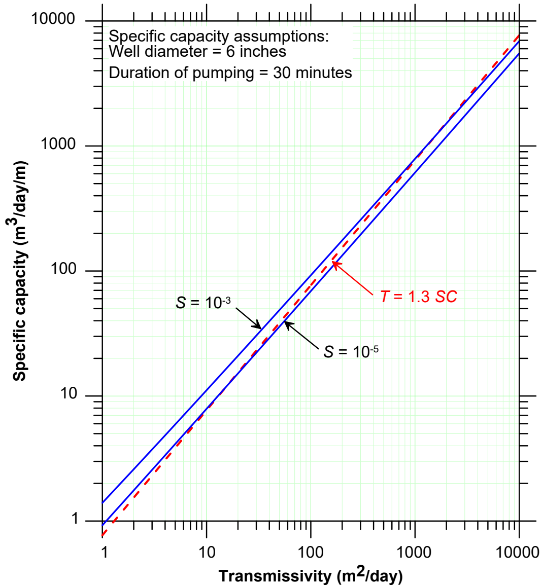
Figure 11. Specific capacity-transmissivity relation, with suggested correlation
