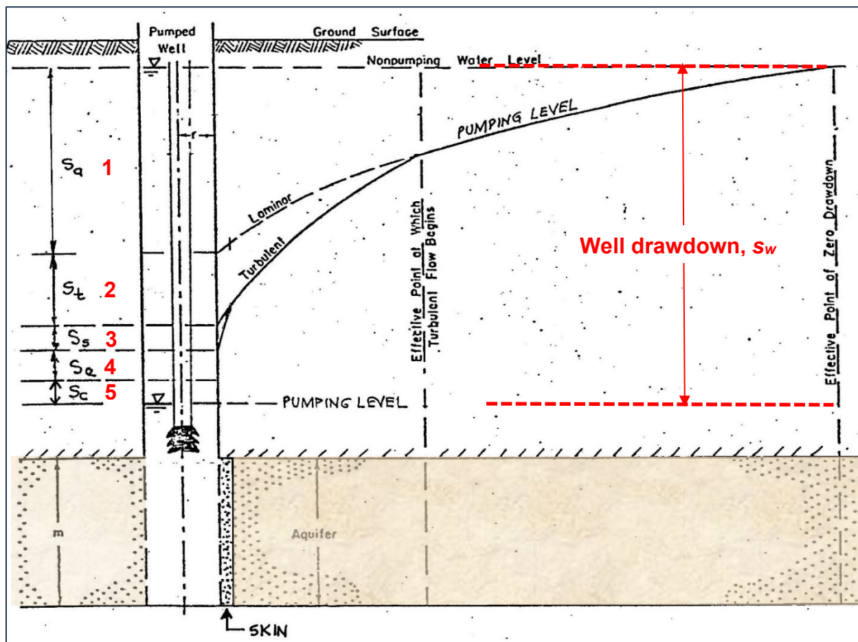
Figure 2. Components of drawdown in a pumping well
