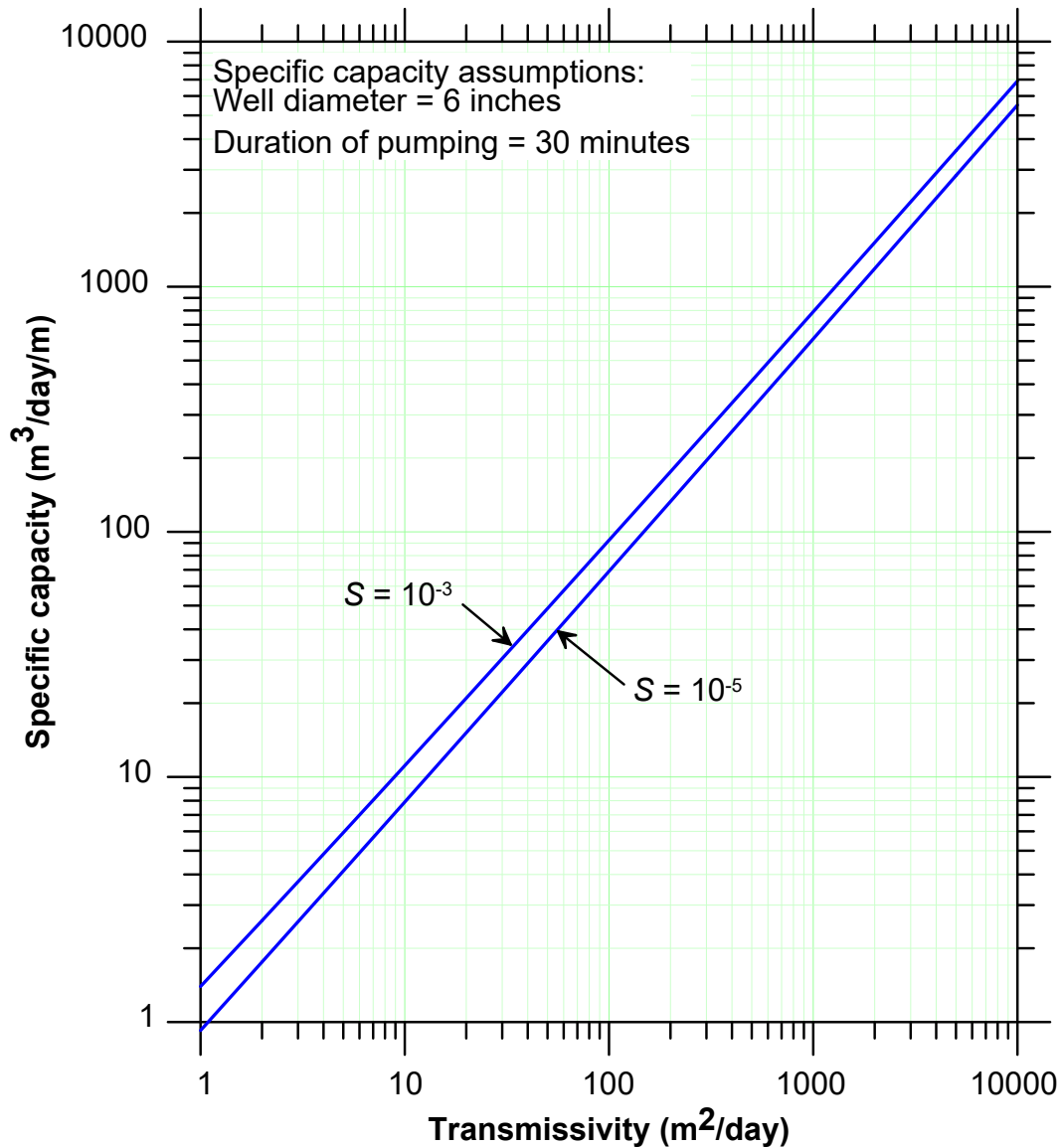
Figure 10. Specific capacity-transmissivity relation
