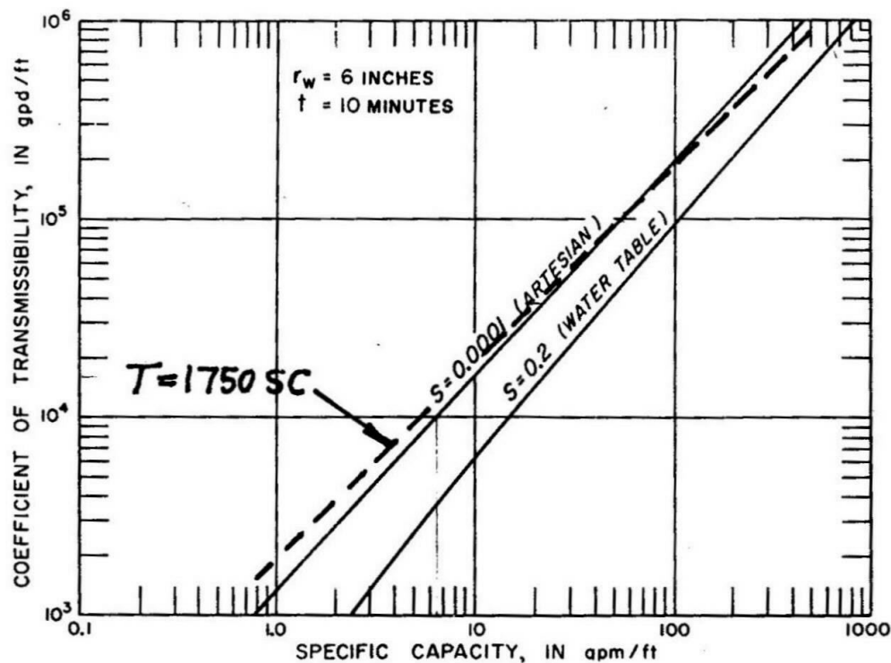
Figure 12. Specific capacity-transmissivity relation for brief pumping
