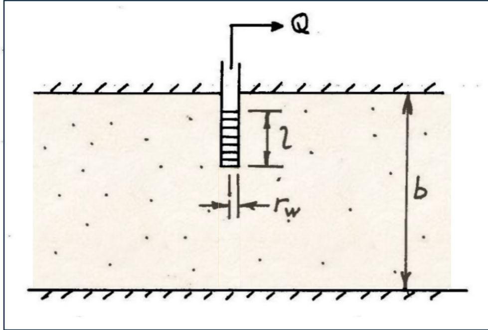
Figure 16. Conceptual model for a partially penetrating well
